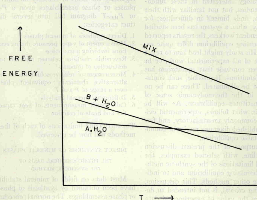
FIG. 1.—Possible free-energy relations between a reactive oxide mix and two crystallization products A \cdot \text{H}_2\text{O} and B at constant pressure. The intersection of the lower lines occurs at the equilibrium temperature of the reaction A \cdot \text{H}_2\text{O} \rightarrow B + \text{H}_2\text{O} . Data in table 1 provide some indication of the separation of these curves.
